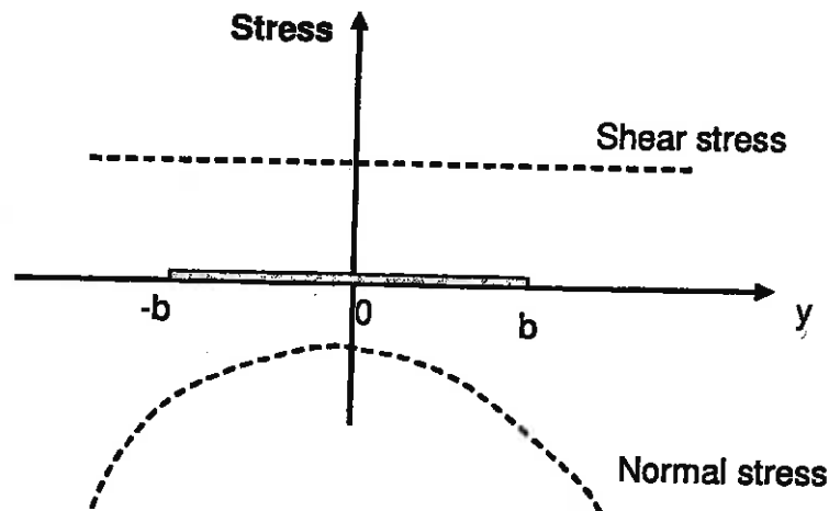
Figure 1: Stress components acting on a fault discontinuity.
