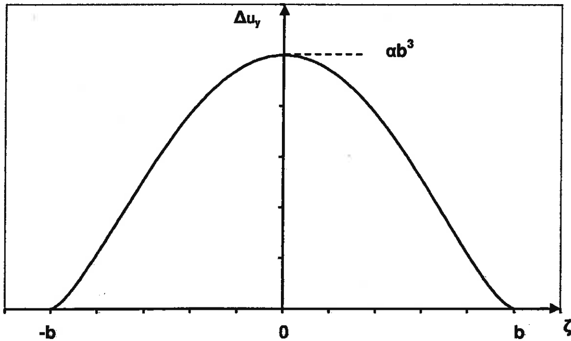
Figure 2: Assumed discontinuity slip profile shape.
