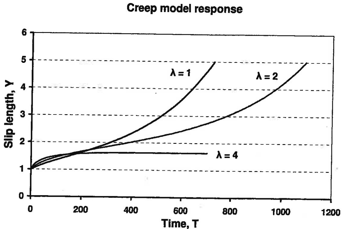
Figure 3: Explicit evolution of the non-dimensional fault activation length, Y , for three values of the critical stability parameter \lambda .
